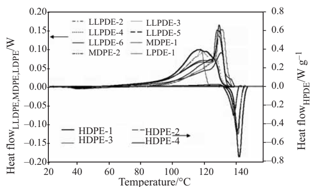
Fig. 6 MDSC non-reversible heat flow
